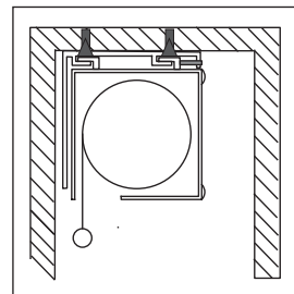
Pelmet Mount
