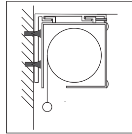
Wall Mount
