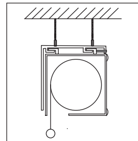
Ceiling Suspension
