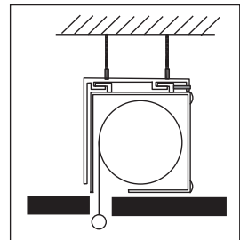
Ceiling Recessed
